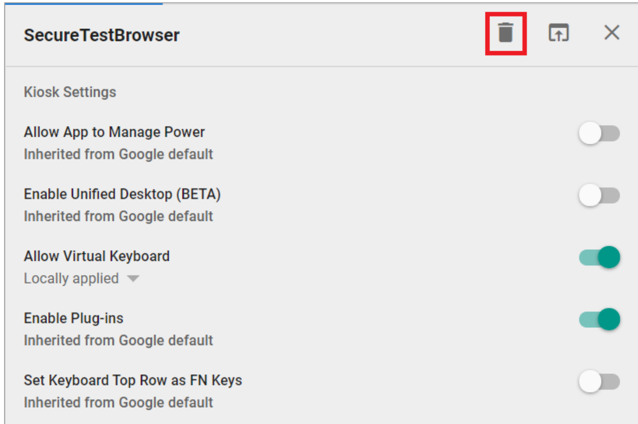
Figure 6. App Settings
